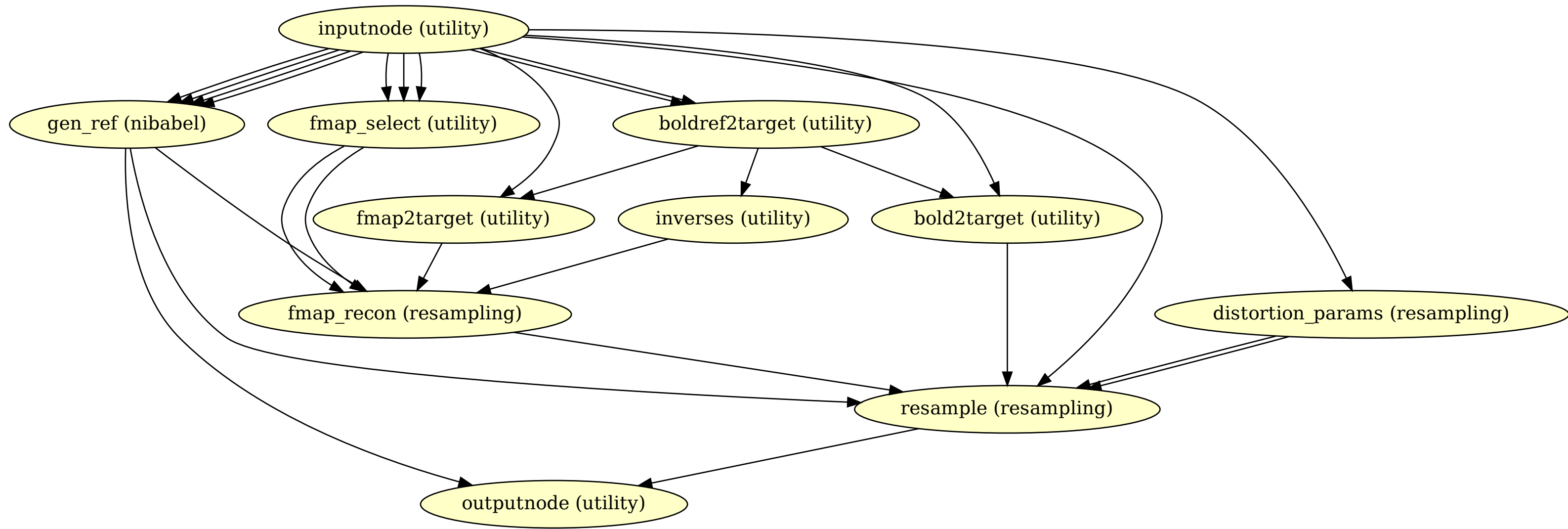
bold_volumetric_resample_wf
