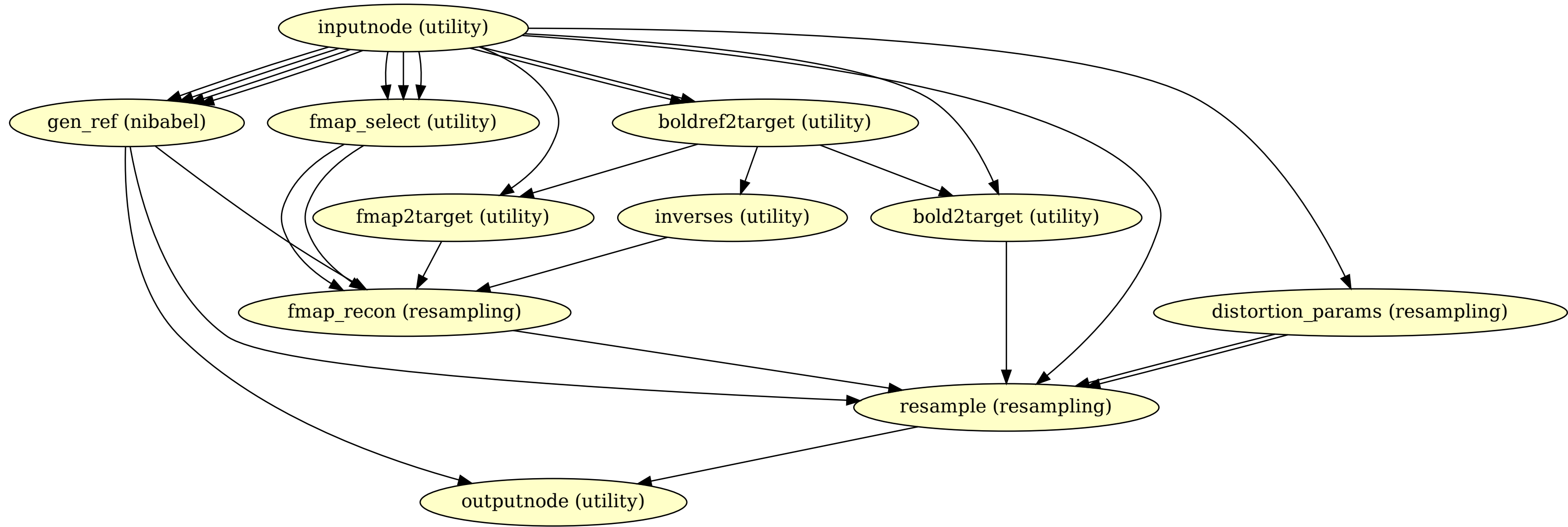
bold_volumetric_resample_wf
